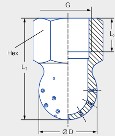
Female thread
