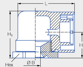
Type 302.606.51.KB
