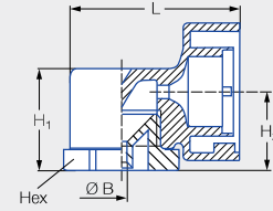
Type 302.32x-302.54x
