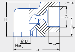
Type 302.32x-302.48x
