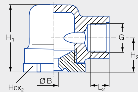
Type 302.52x-302.96x
