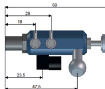
Part no. 1080720000
