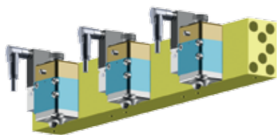
Example of individual BS 25-SRV-15 Mini nozzle bar with medium block 50 mm
