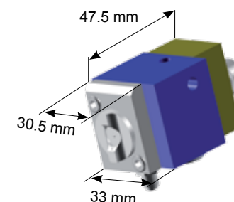
ST block nozzle CD-100 BSD
