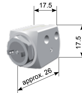
CD 105 block nozzle
