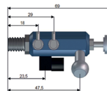
Part no. 1080720088
