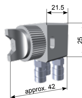
CD 95 block nozzle
