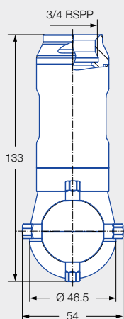
Female thread 5TA.403.1Y.AL and 5TA.404.1Y.AL
