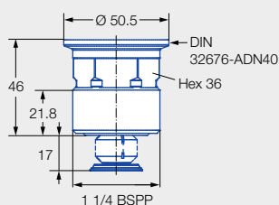
Male thread
