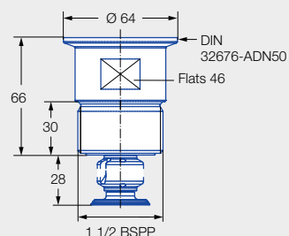
Male thread
