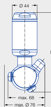
Female thread
