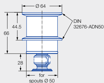
Tri-Clamp connection 2
