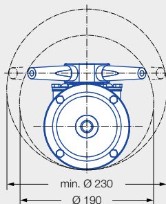
5TM.4xx.1Y.AS (4 nozzles)
