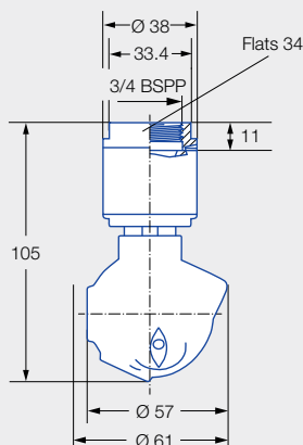
Female thread
