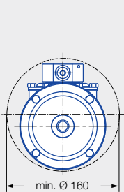
5TM.2xx.1Y.AS (2 nozzles)
