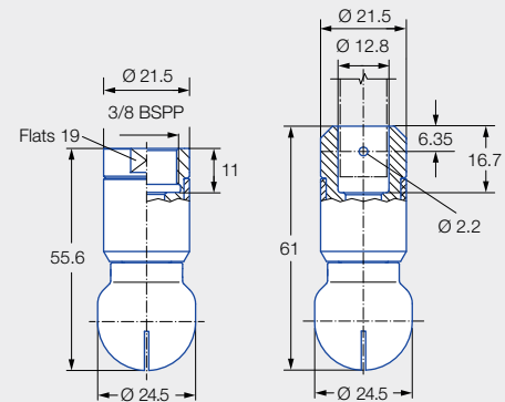
Female thread
