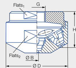
130° version
