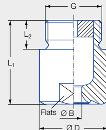
120° version
