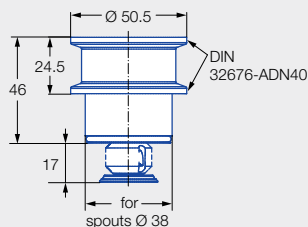
Tri-Clamp connection 1
