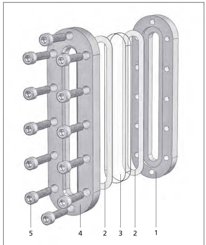
Exploded view of an oblong oval sight glass fitting
